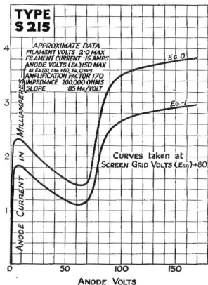
Characteristic Curve of Average S 215 Valve.
